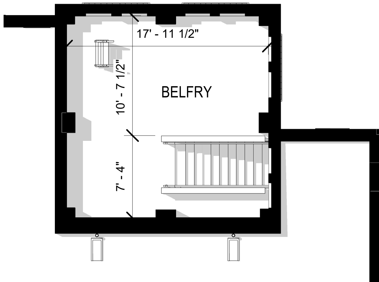
THE CHURCH STUDIO BELFRY (NOT TO SCALE)
